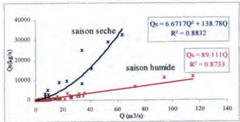
Fig. 8 - Relation débit solide-débit liquide station L.O. Farés (1983/2001)
