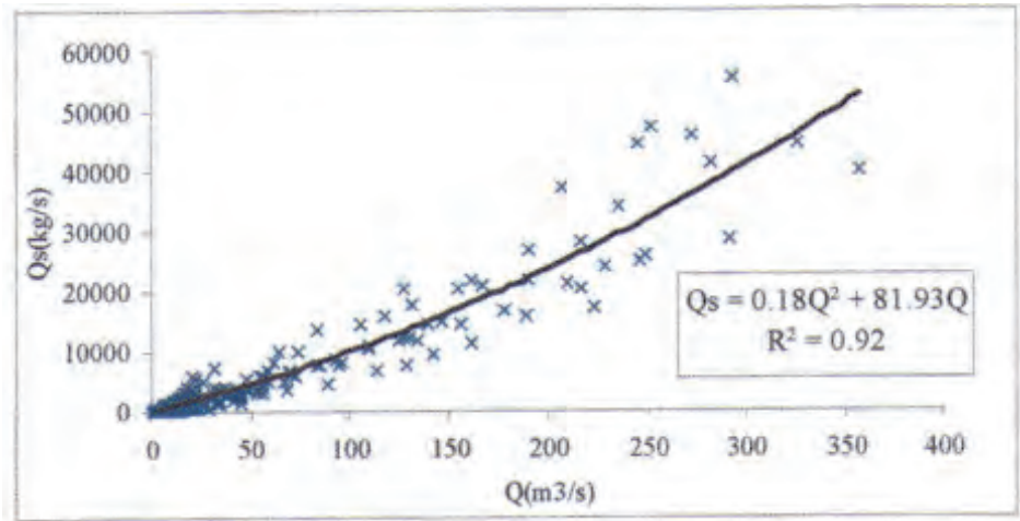
Fig. 7 - Relation débit solide-débit liquide station S.Akkacha (1983/2001)
