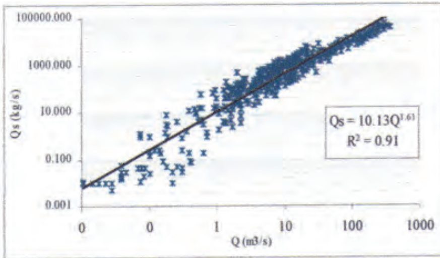
Fig. 5 - Relation débit liquide-débit solide station S.Akkacha 'O.Allala
